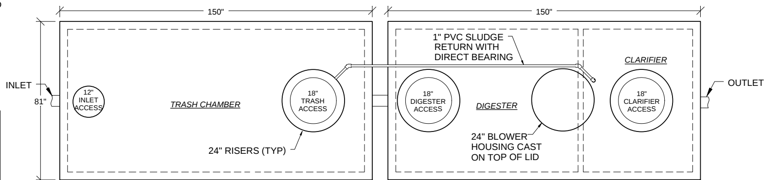
BNR-1500 TOP VIEW NO SCALE
