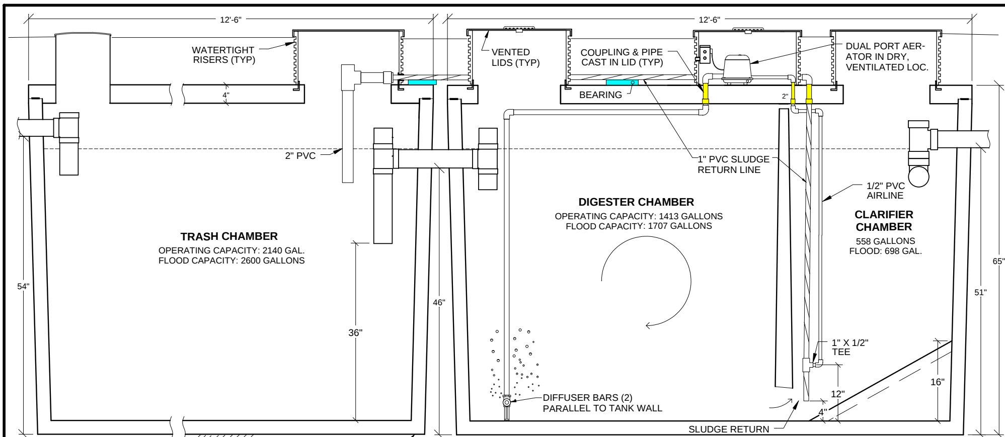
BNR-1500 SIDE VIEW NO SCALE
