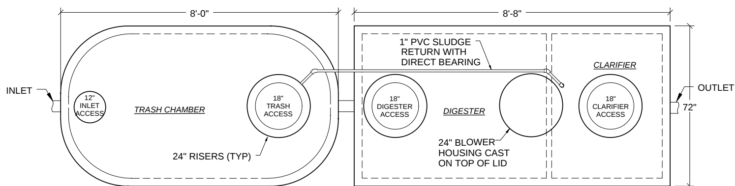
BNR-1000 TOP VIEW NO SCALE
