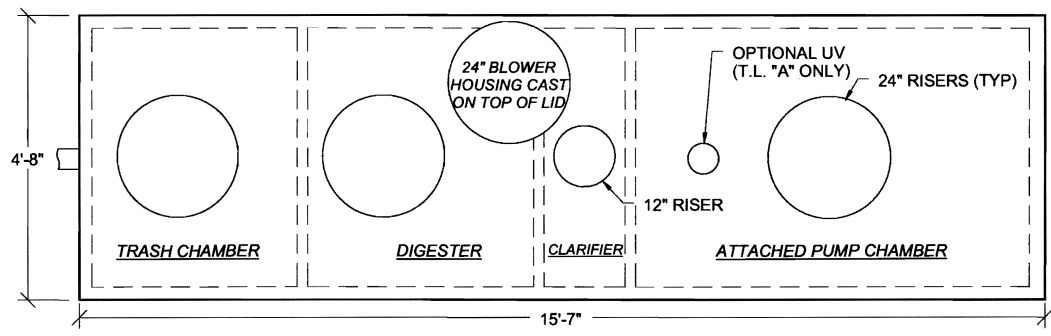
NuWATER ATU COMBO TANK DETAIL FOR MODEL BNR-500 TREATMENT UNIT REVISED: 3/1/12
