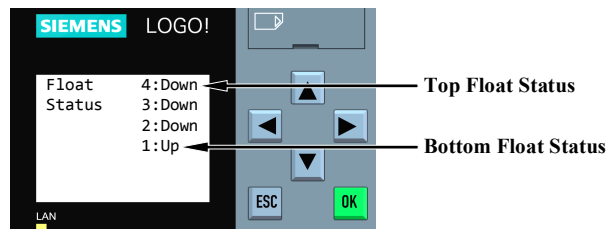
Figure 1. Float Status and Timer Mode Screen
