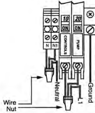
One Circuit
