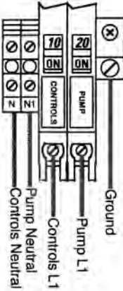
Two Circuits
